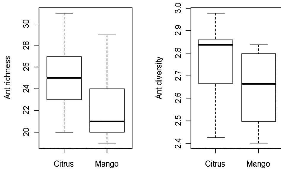
Fig. 3. Variation in ant richness and ant diversity depending on the main crop in the type 3 and type 4 orchards located in the localities of Ndoienne and Notto. Citrus orchards were continuously irrigated and mango orchards were only irrigated for five months (January–May).
