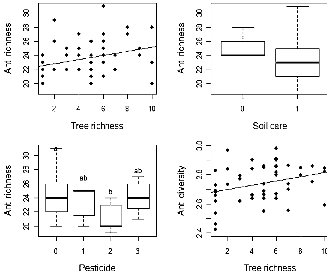
Fig. 4. Relations between ant richness, ant diversity and two variables relative to orchard design (tree richness) and management practices (soil care: 0 = no soil care, 1 = shallow tillage and/or mechanical weeding of soil; pesticide: 0 = no pesticide, 1 = 1–2 applications per year, 2 = 3–5 applications per year, 3 = more than 5 applications per year).
